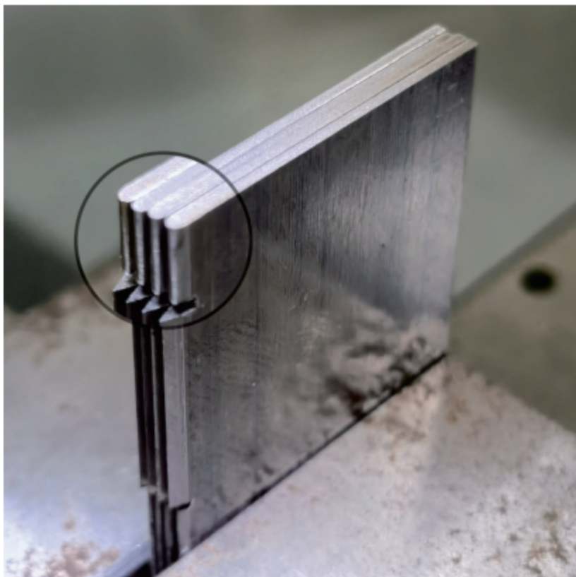
刀线组合端面磨圆角 Cut Crease Side Grinding
